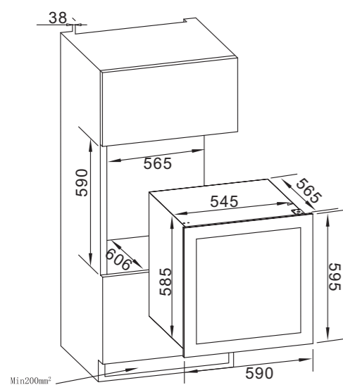
Installation drawing
